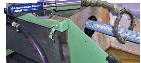
PVC hose is cooled at the exit of an extruder so it can be coiled immediately.
