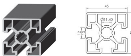
Perfil 45x45 3S Profile 45x45 3S
