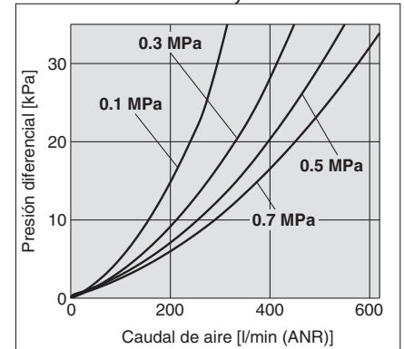
ZFC76/7F Ø 10, Ø 3/8"
