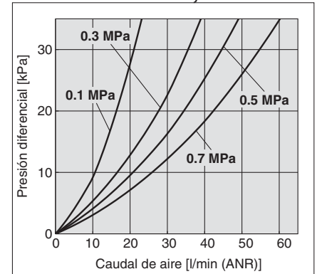
ZFC32/3A Ø 3.2, Ø 1/8"
