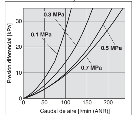
ZFC54/5D Ø 6, Ø 1/4"
